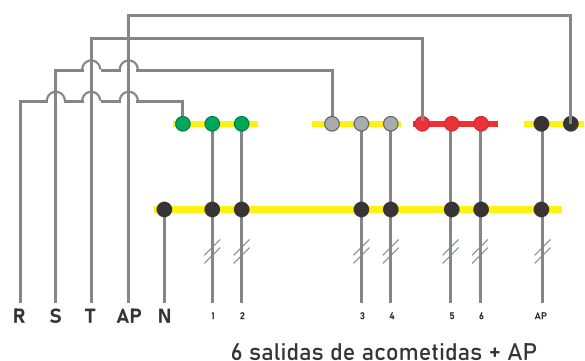
Diagrama Unifilar CDBS 380-220V 6S +1AP
