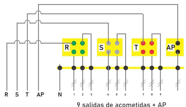
Diagrama unifilar CDBS 380-220V 9S +1AP
